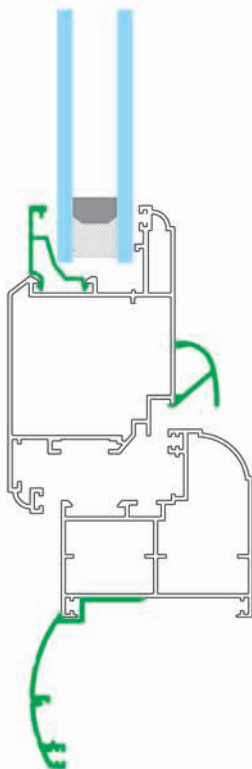
Section A
