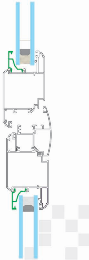
Section B
